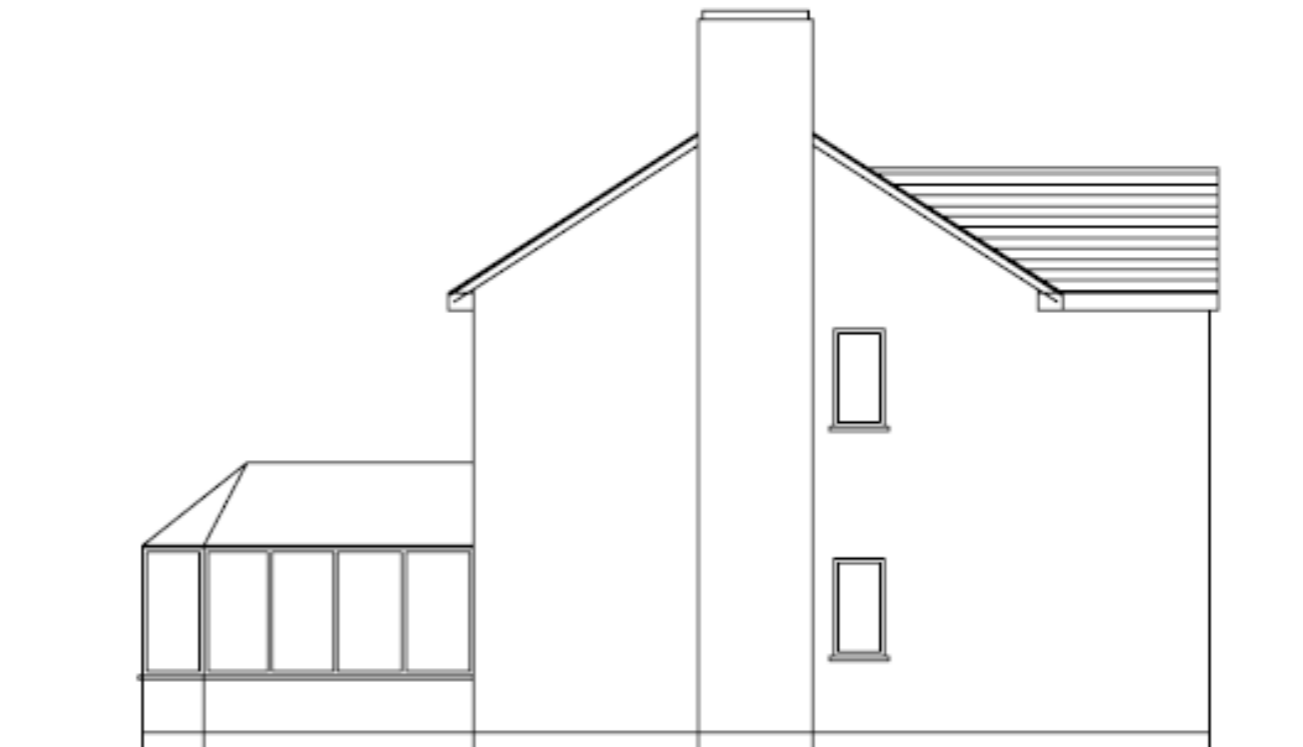
PRE EXISTING WEST SIDE ELEVATION
